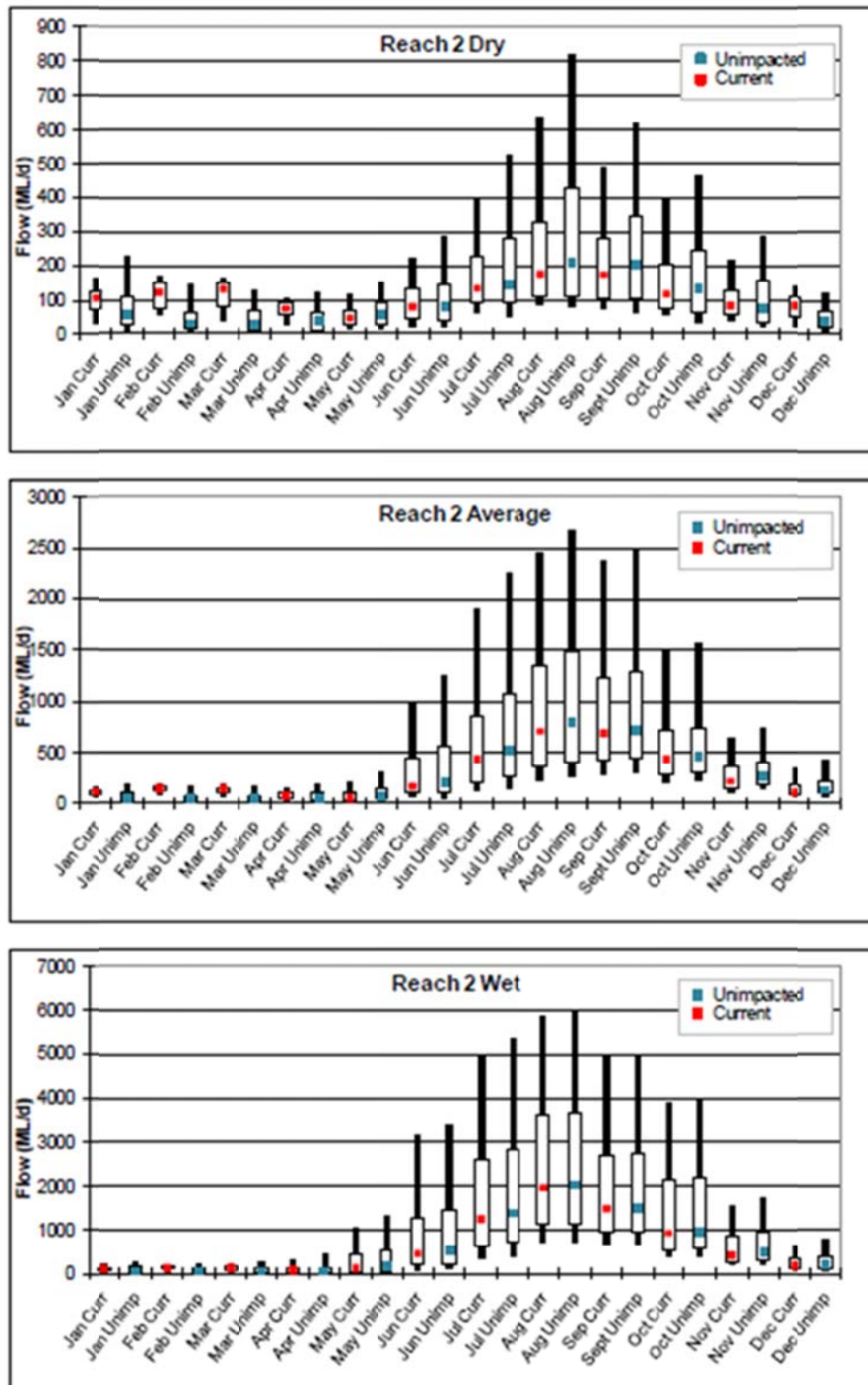
Figure 8: Plots of mean daily flow for each month in dry, average and wet years in Reach 2.
