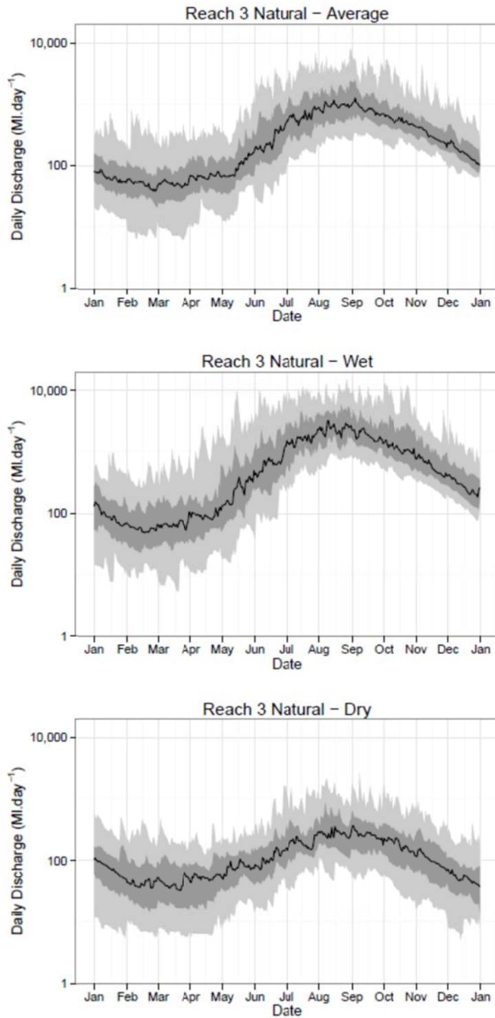
Figure 13: Reach 3 natural flows for average, wet and dry scenarios. Black line = median; dark grey = 20 th – 80 th percentile flows; light grey = 5 th – 95 th percentile flows.
