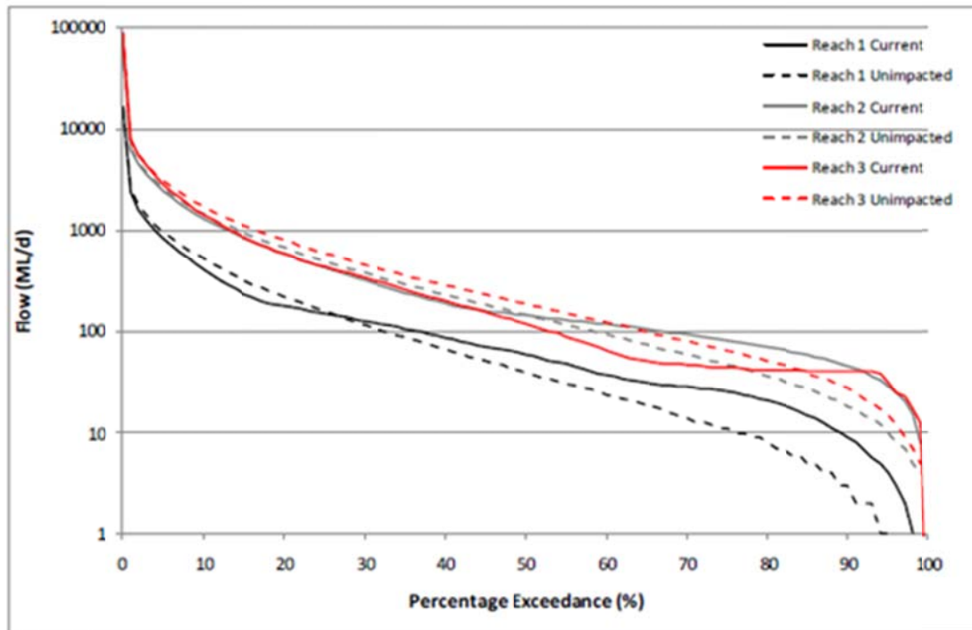
Figure 3: Flow duration curves for the modelled current and unregulated flow series in Reaches 1-3.
