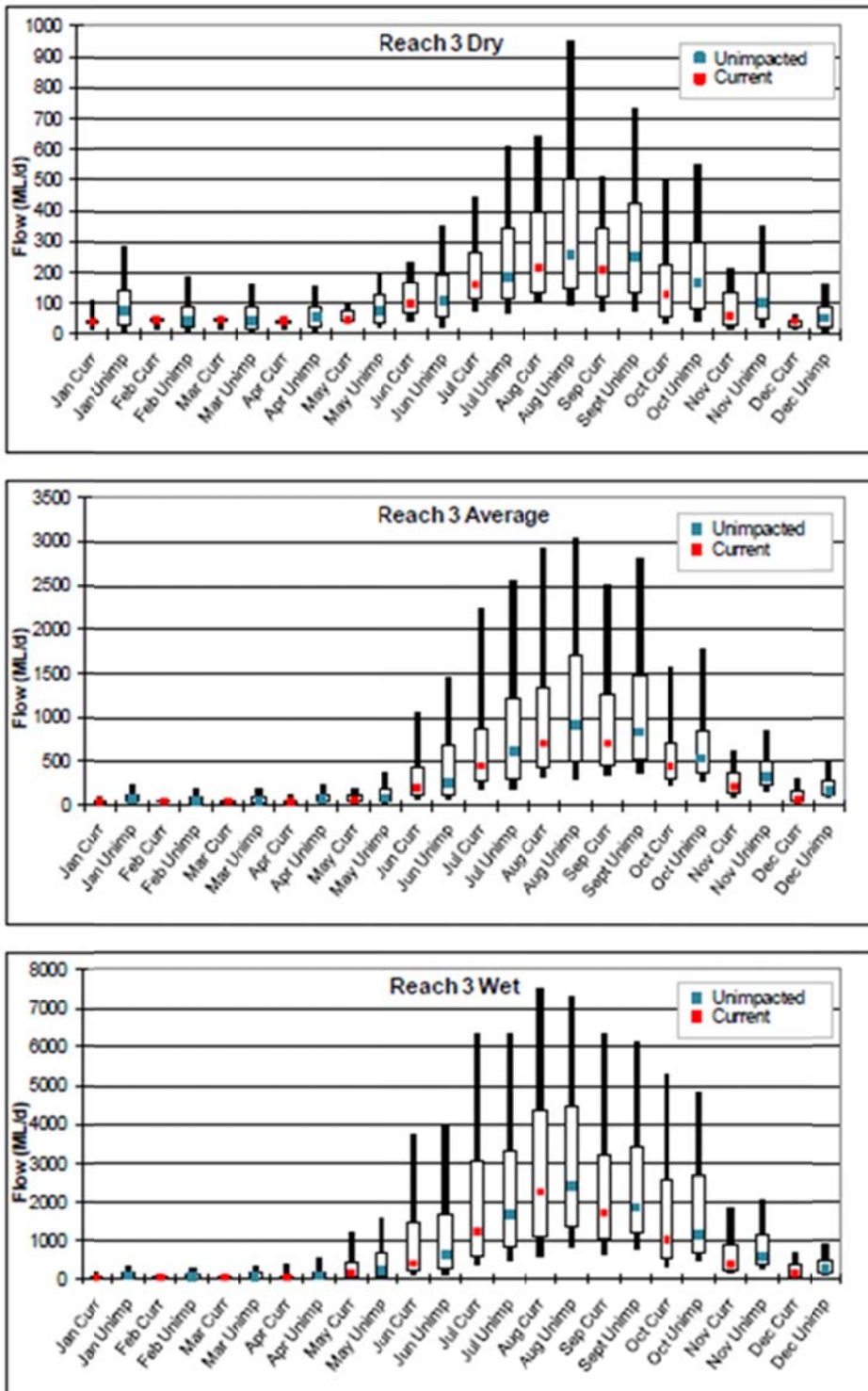
Figure 9: Plots of mean daily flow for each month in dry, average and wet years in Reach 3.
