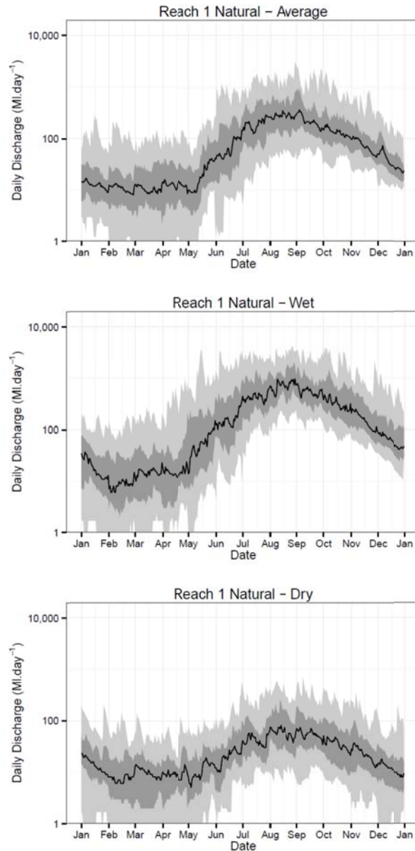
Figure 11: Reach 1 natural flow for average, wet and dry scenarios. Black line = median; dark grey = 20 th – 80 th percentile flows; light grey = 5 th – 95 th percentile flows.
