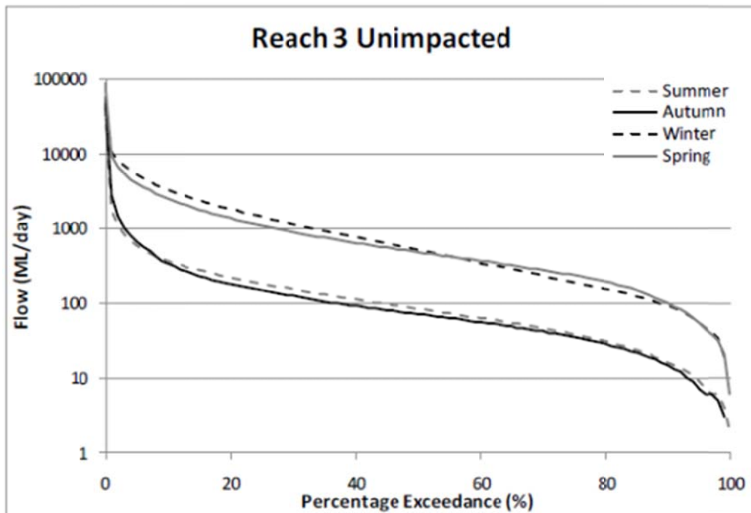
Figure 6: Flow duration curves showing seasonal patterns for modelled current and unregulated conditions.
