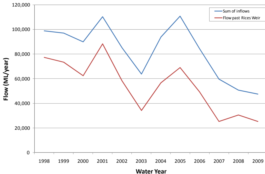
Figure 7-8 A comparison of annual total inflows (including from the upstream catchments, outfalls and drains) and annual flow past Rices Weir (some data infilled as outlined in Appendix D) up to 2009
