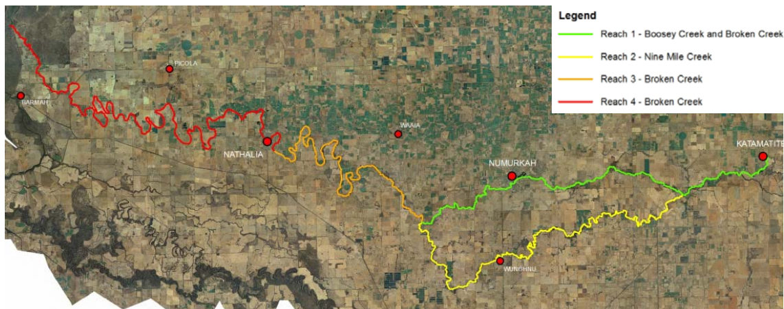
Figure 4-2 EWP project area and project reaches
