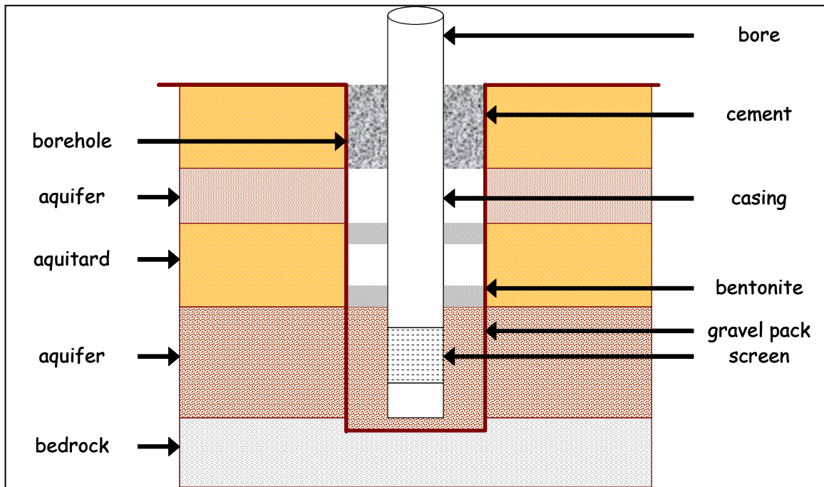
Figure 17: Example Bore Construction
