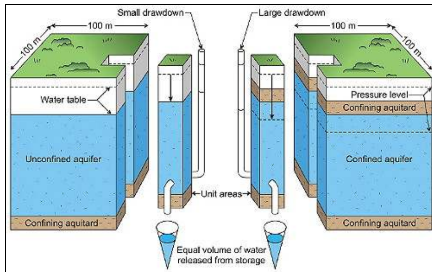
Figure 8 Larger drawdown in confined aquifer compared to unconfined aquifer
