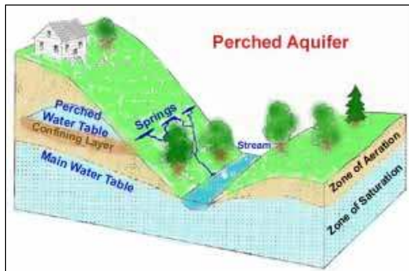
Figure 4 Perched aquifer (source: http://www.co.pepin.wi.us )
