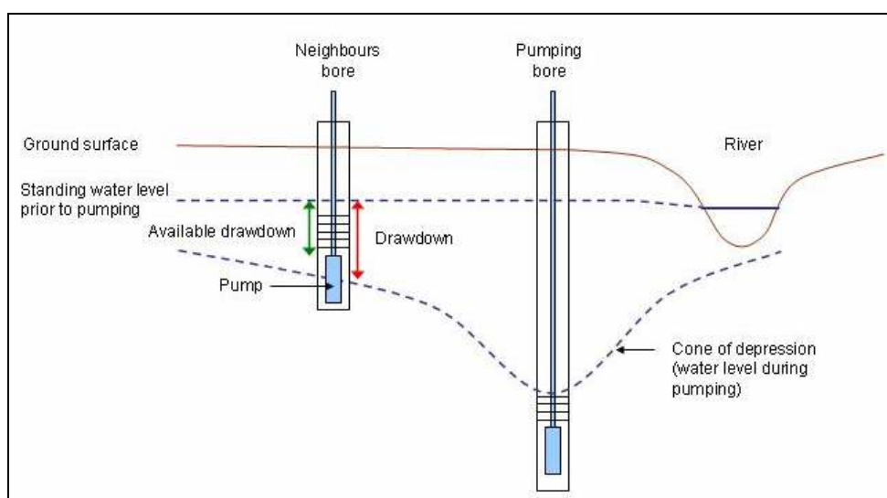
Figure 18: Pumping interference to neighbouring bore and stream
