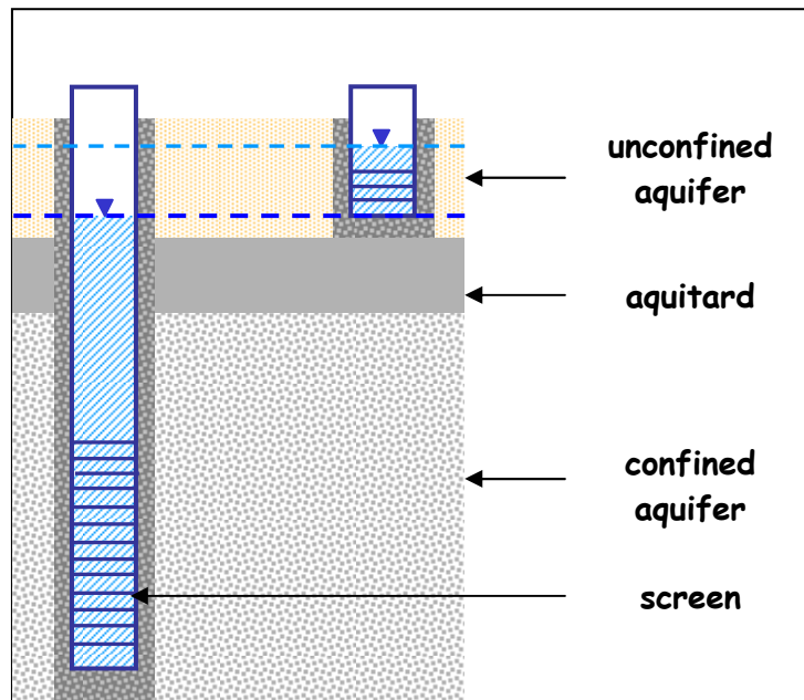
Figure 21 Nested monitoring bores in cross-section
