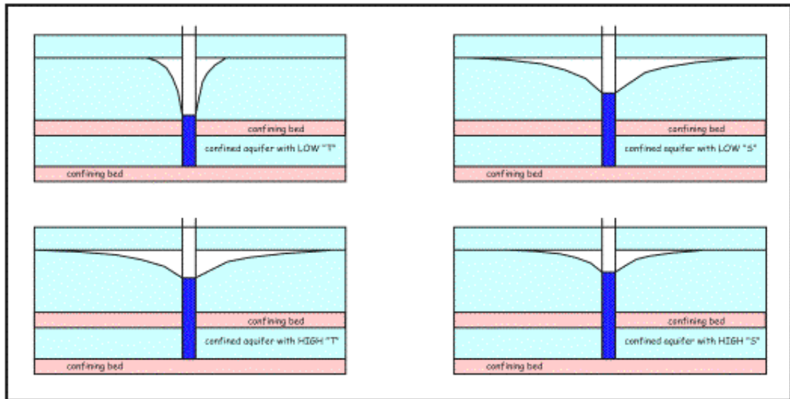
Figure 16 Cone of depression for various aquifer characteristics
