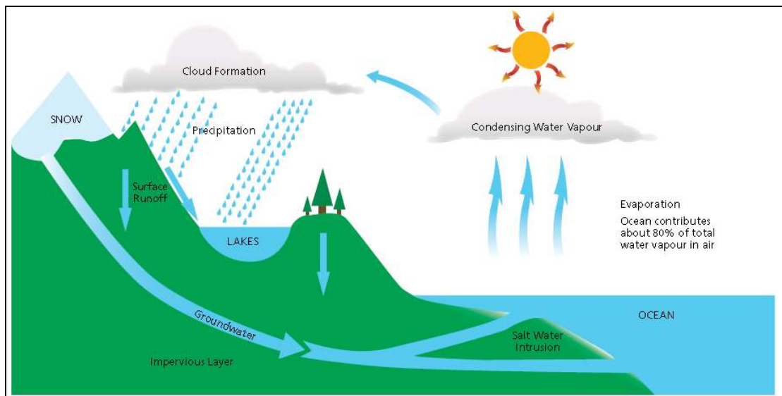
Figure 1: Water Cycle (source: Department of Sustainability and Environment Groundwater Notes 1 February 2009)
