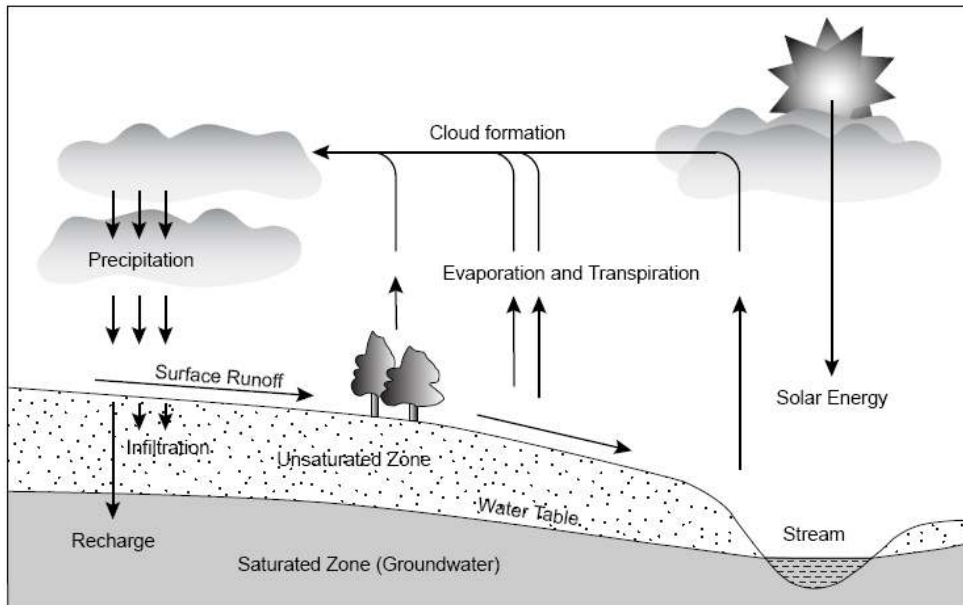
Figure 10 Groundwater recharge to unconfined aquifer
