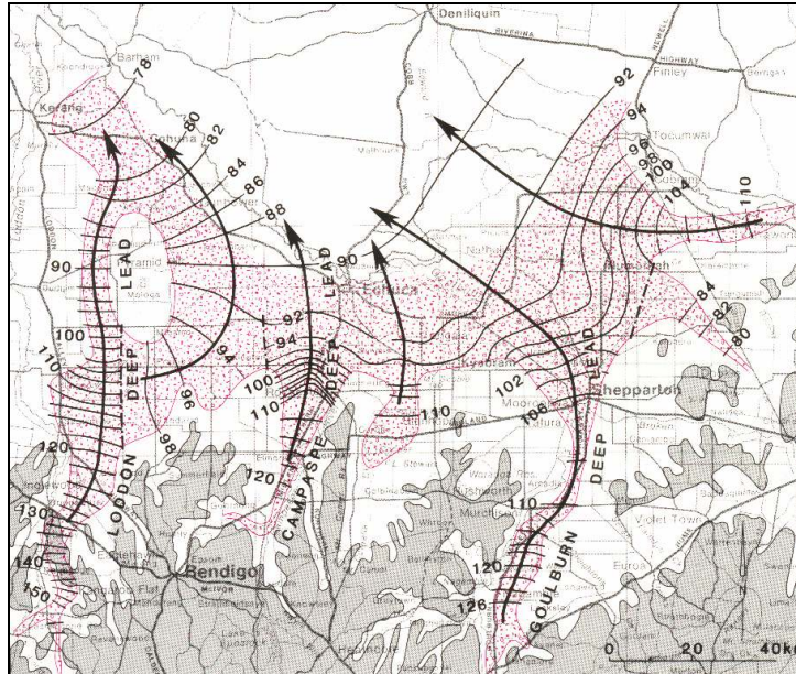
Figure 24: Potentiometric surface of the deep lead system of Northern Victoria – August 1981 illustrating northward groundwater flow (source: Macumber, 1991).
