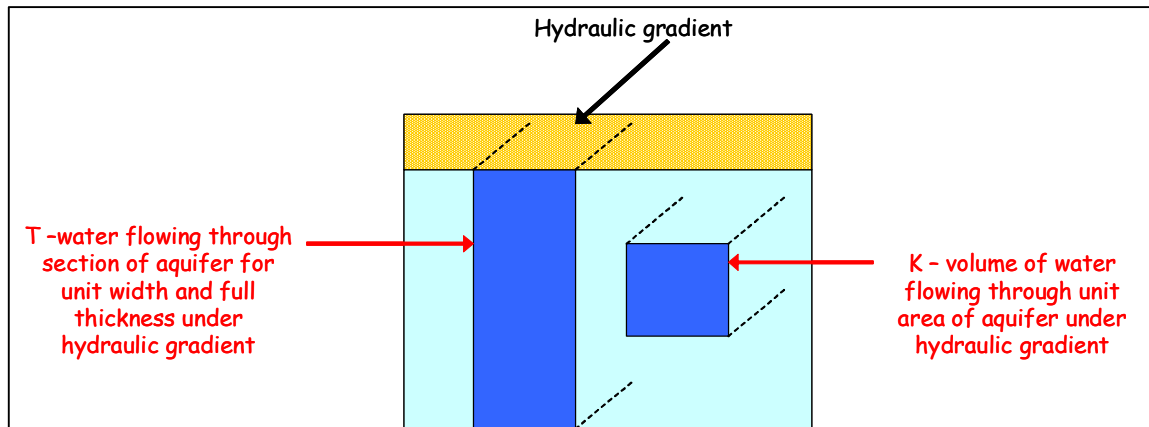
Figure 7 Aquifer transmissivity and hydraulic conductivity (source: http://www.ncwater.org )
