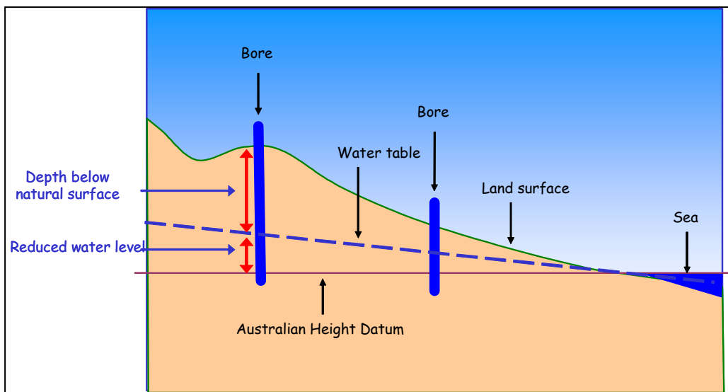
Figure 5 Measures of groundwater level depth below natural surface and against the Australian height datum
