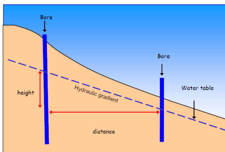
Figure 6: Hydraulic gradient slope between two bores
