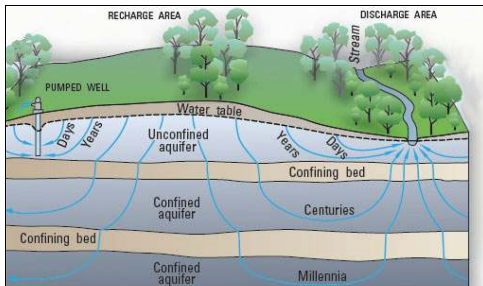
Figure 9 Groundwater flow (source: http://www.usgs.gov/ )
