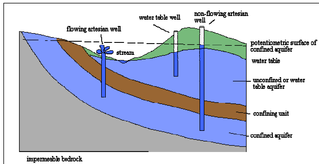
Figure 3 Aquifer types (source: https://netfiles.uiuc.edu )
