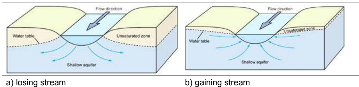
Figure 13: surface water-groundwater interactions (source: Winter et al. 1989)
